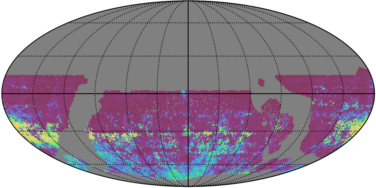
ddf_acor_sf10_lsf40_lsr50_v3.4_10yrs WFD r band: 75th Percentile Intranight Timespan
