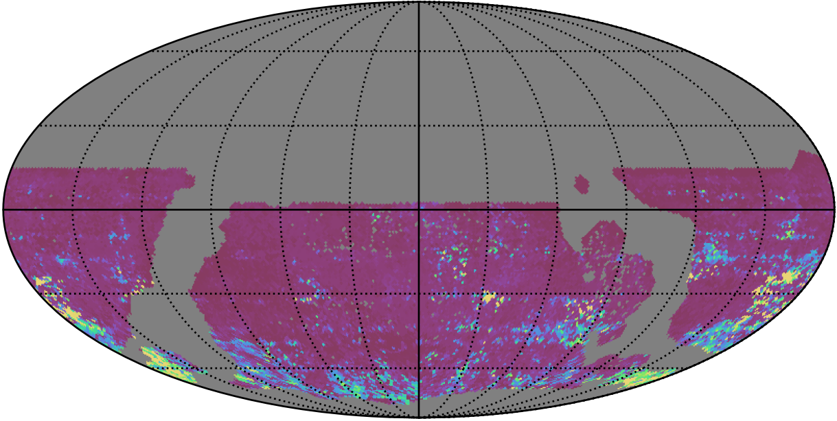
ddf_acor_sf10_lsf40_lsr50_v3.4_10yrs WFD i band: 75th Percentile Intranight Timespan
