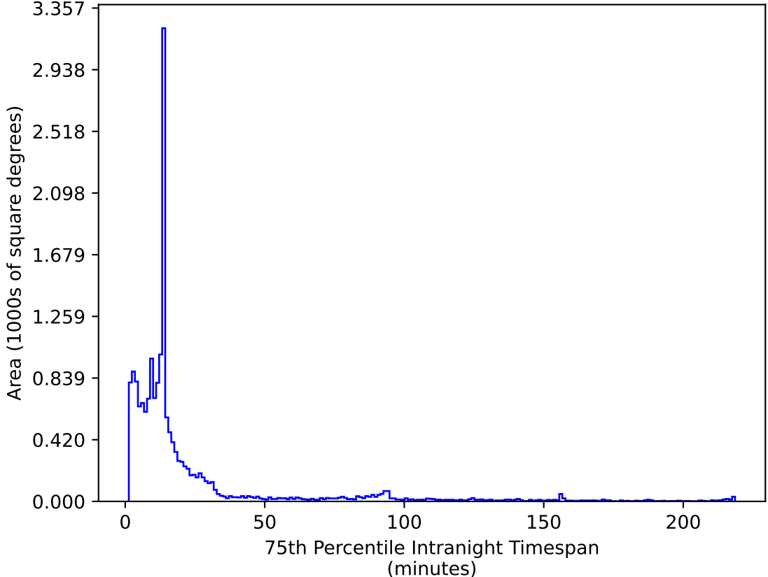
ddf_acor_sf10_lsf40_lsr50_v3.4_10yrs WFD i band: 75th Percentile Intranight Timespan
