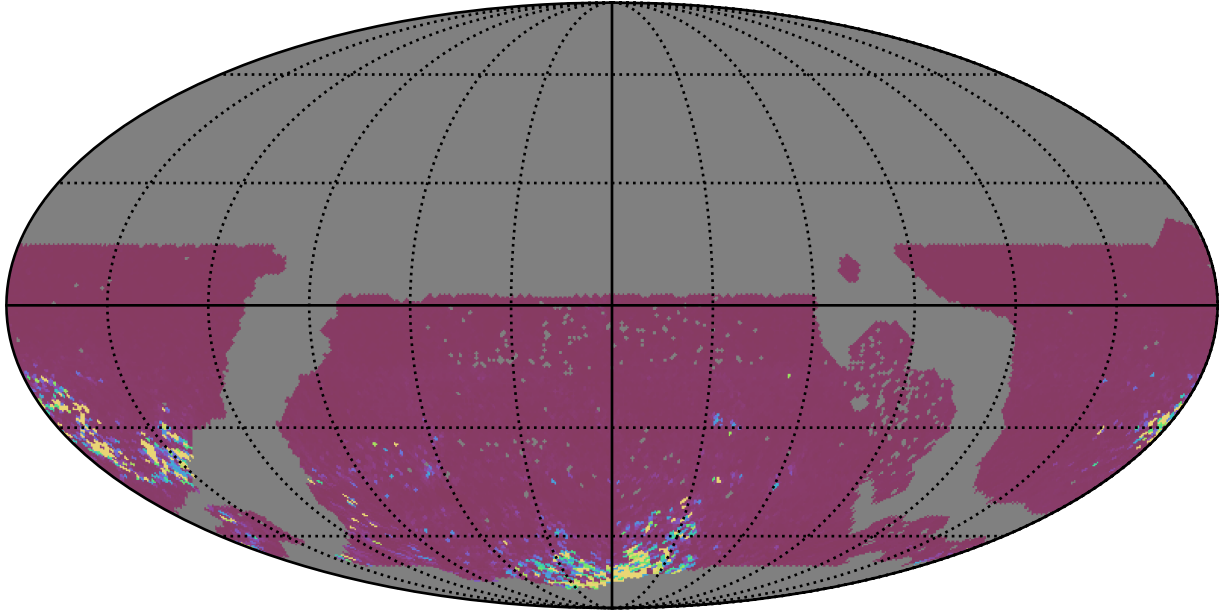
ddf_acor_sf10_lsf40_lsr50_v3.4_10yrs WFD gr bands: 75th Percentile Intranight Timespan
