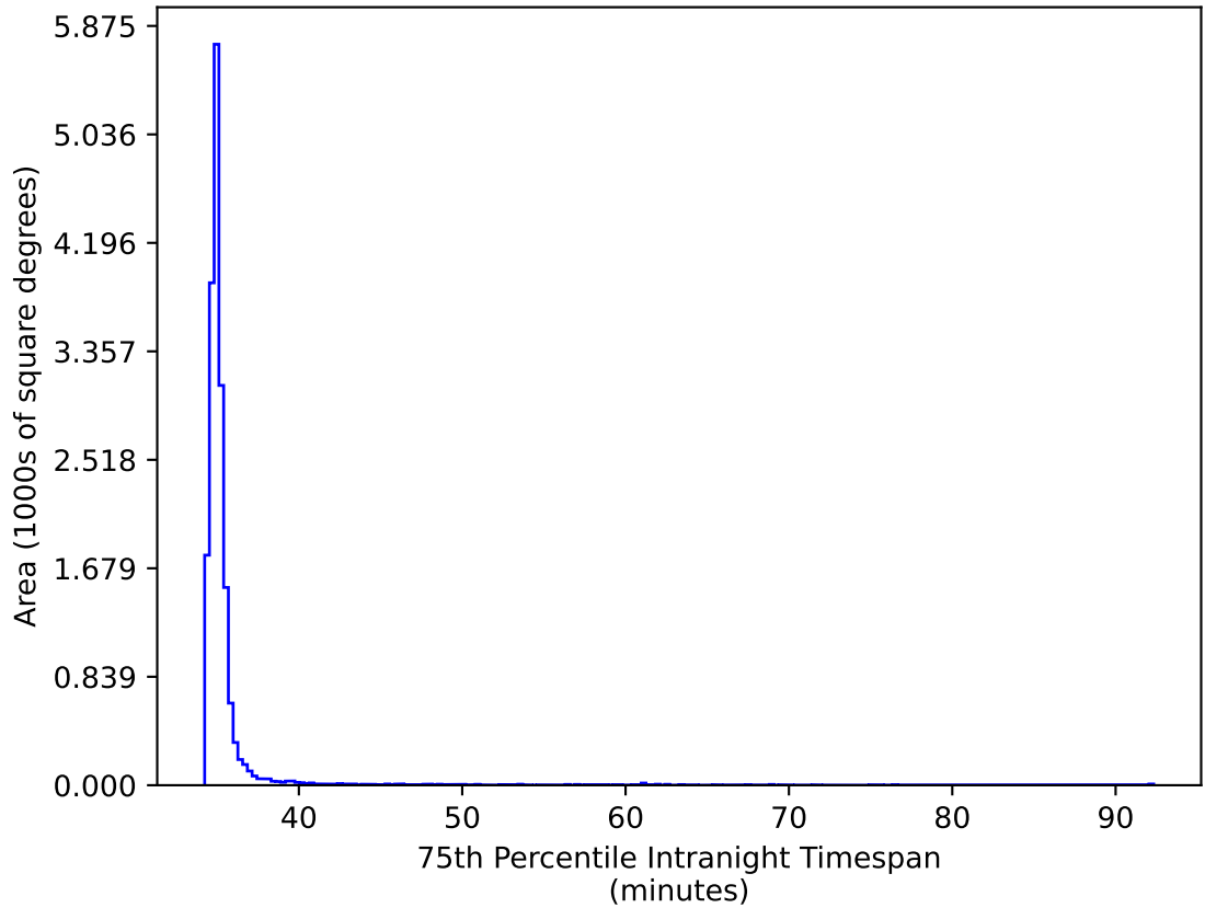
ddf_acor_sf10_lsf40_lsr50_v3.4_10yrs WFD gr bands: 75th Percentile Intranight Timespan
