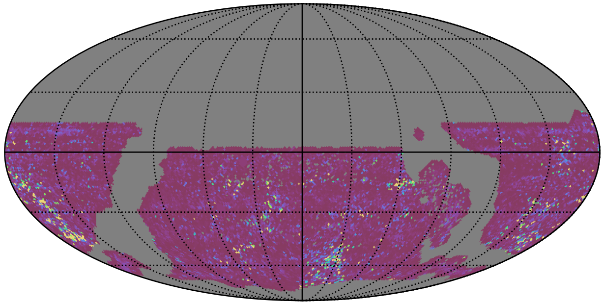
ddf_acor_sf10_lsf40_lsr50_v3.4_10yrs WFD g band: 75th Percentile Intranight Timespan
