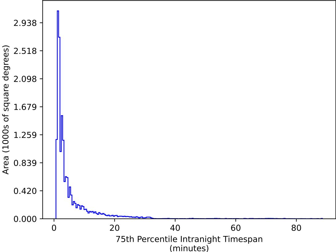
ddf_acor_sf10_lsf40_lsr50_v3.4_10yrs WFD g band: 75th Percentile Intranight Timespan
