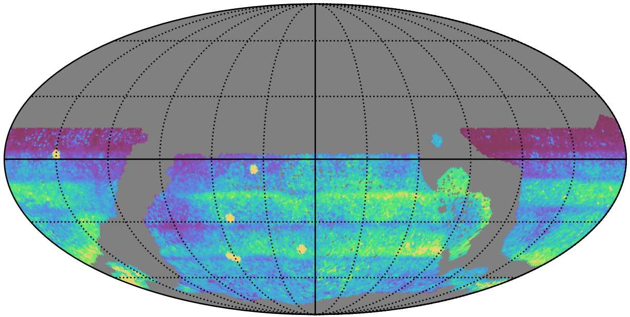
ddf_acor_sf10_lsf40_lsr50_v3.4_10yrs WFD all bands: 75th Percentile Intranight Timespan
