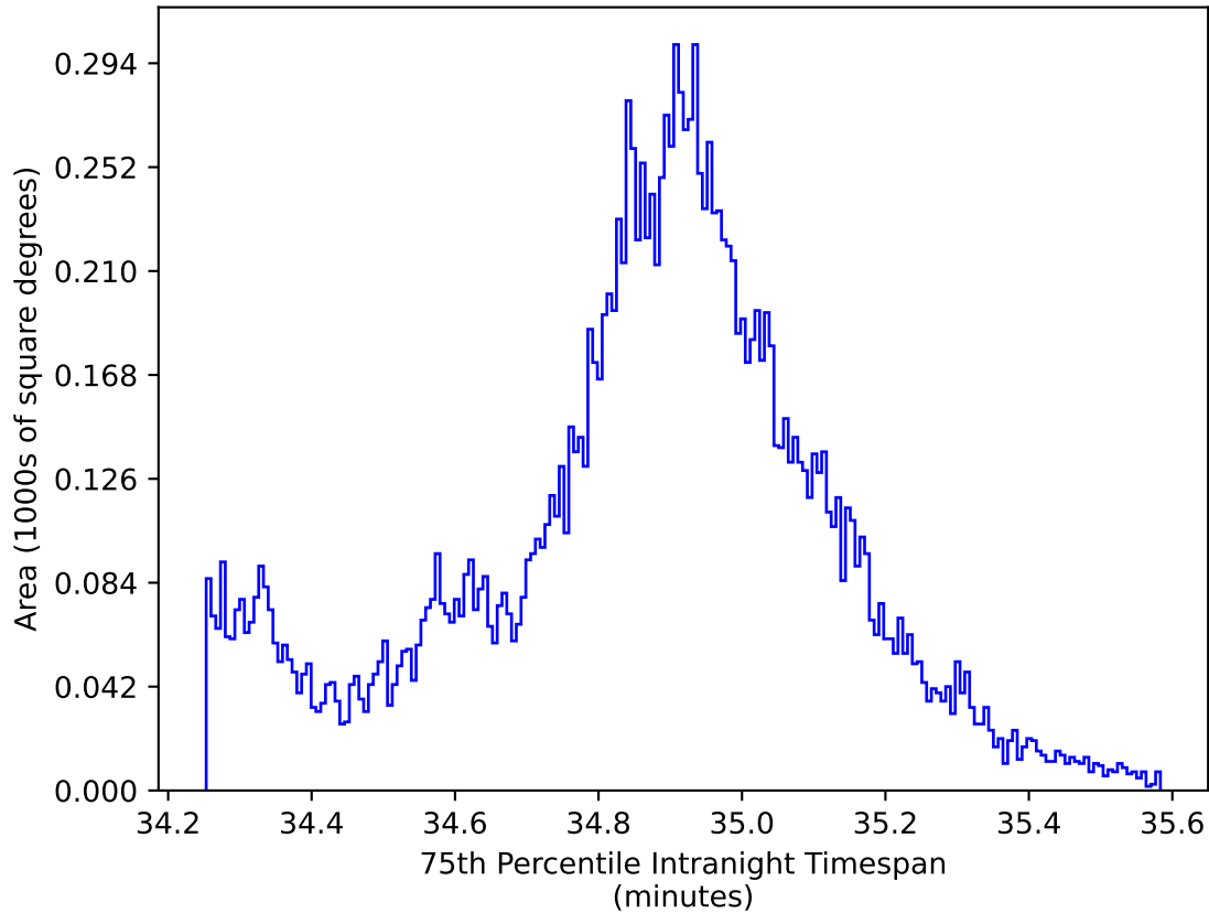
ddf_acor_sf10_ls40_lsr50_v3.4_10yrs WFD: 75th Percentile Intranight Timespan
