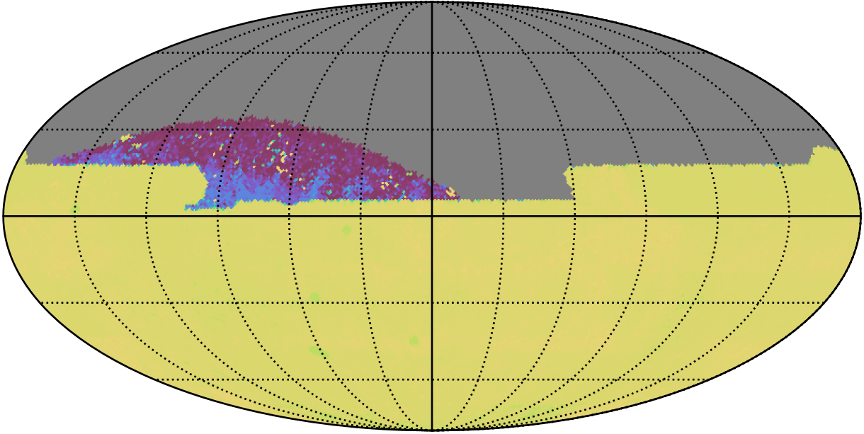
ddf_acor_sf10_lsf40_lsr50_v3.4_10yrs All sky zy bands: 75th Percentile Intranight Timespan
