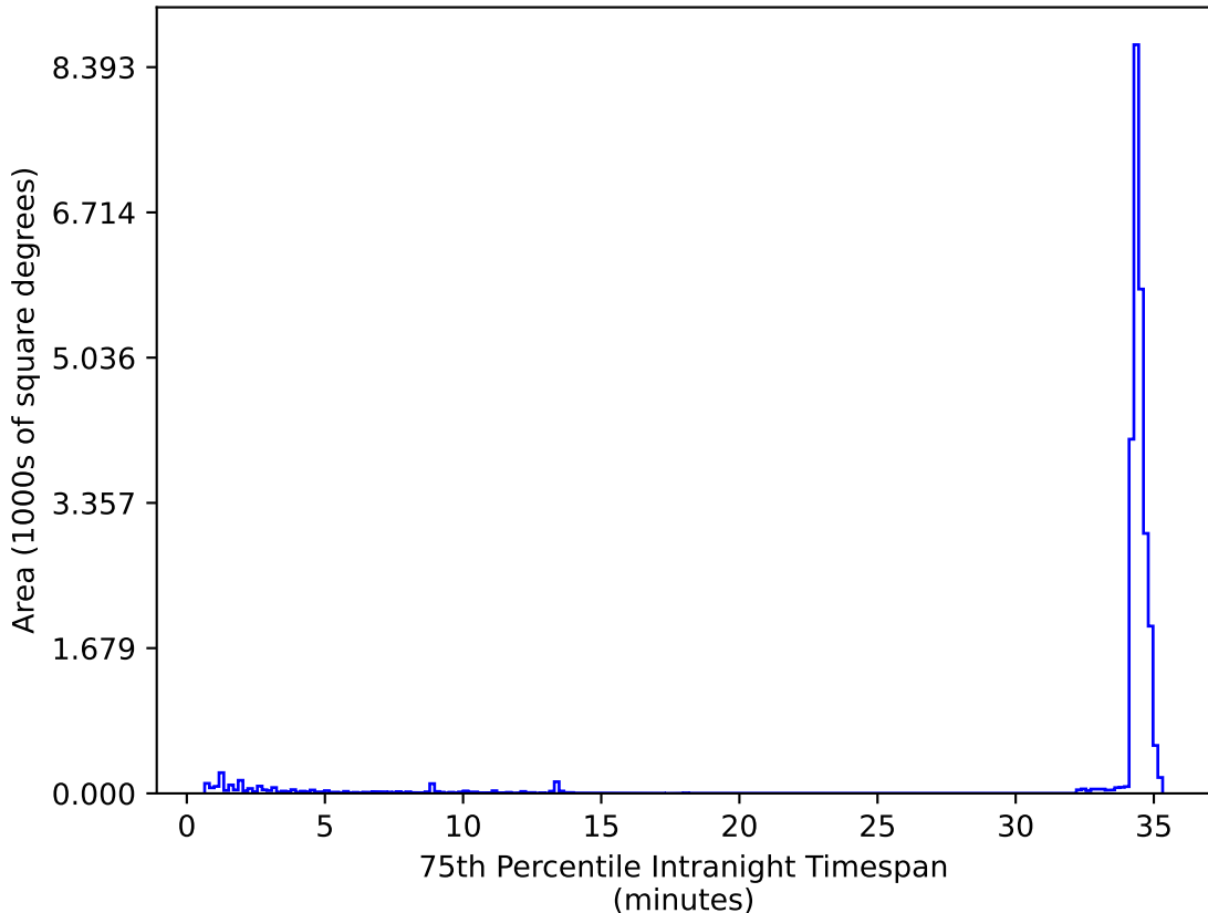
ddf_acor_sf10_lsf40_lsr50_v3.4_10yrs All sky zy bands: 75th Percentile Intranight Timespan
