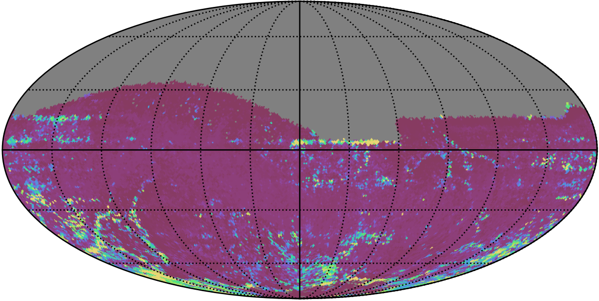
ddf_acor_sf10_lsf40_lsr50_v3.4_10yrs All sky z band: 75th Percentile Intranight Timespan
