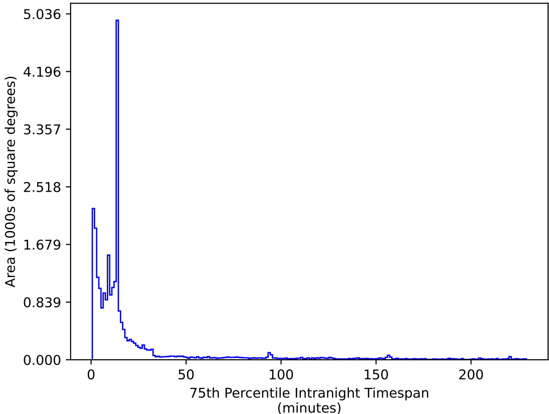
ddf_acor_sf10_lsf40_lsr50_v3.4_10yrs All sky z band: 75th Percentile Intranight Timespan
