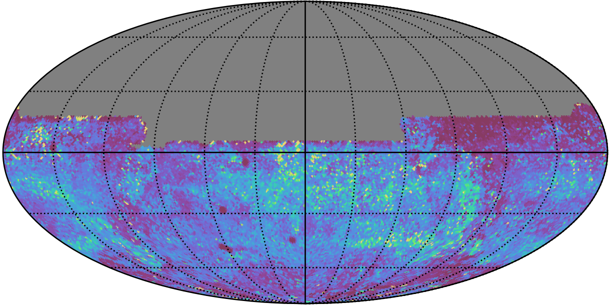
ddf_acor_sf10_lsf40_lsr50_v3.4_10yrs All sky y band: 75th Percentile Intranight Timespan
