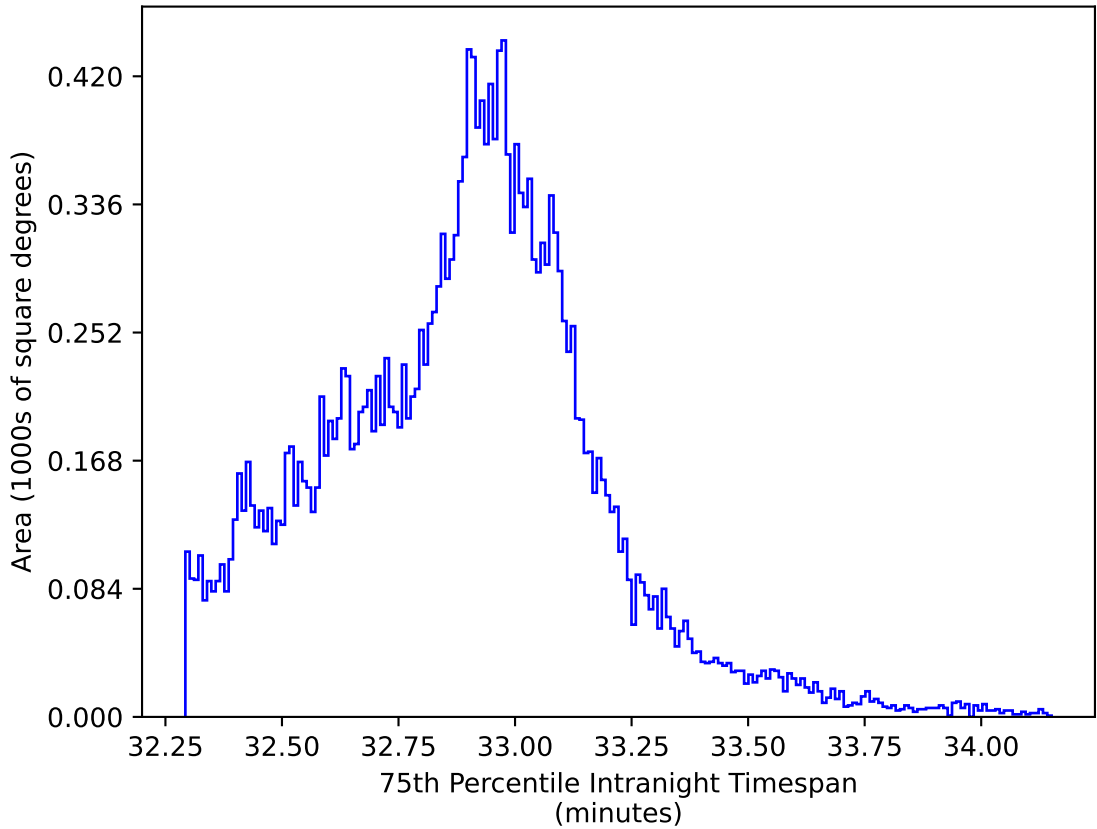
ddf_acor_sf10_ls40_lsr50_v3.4_10yrs All sky y band: 75th Percentile Intranight Timespan
