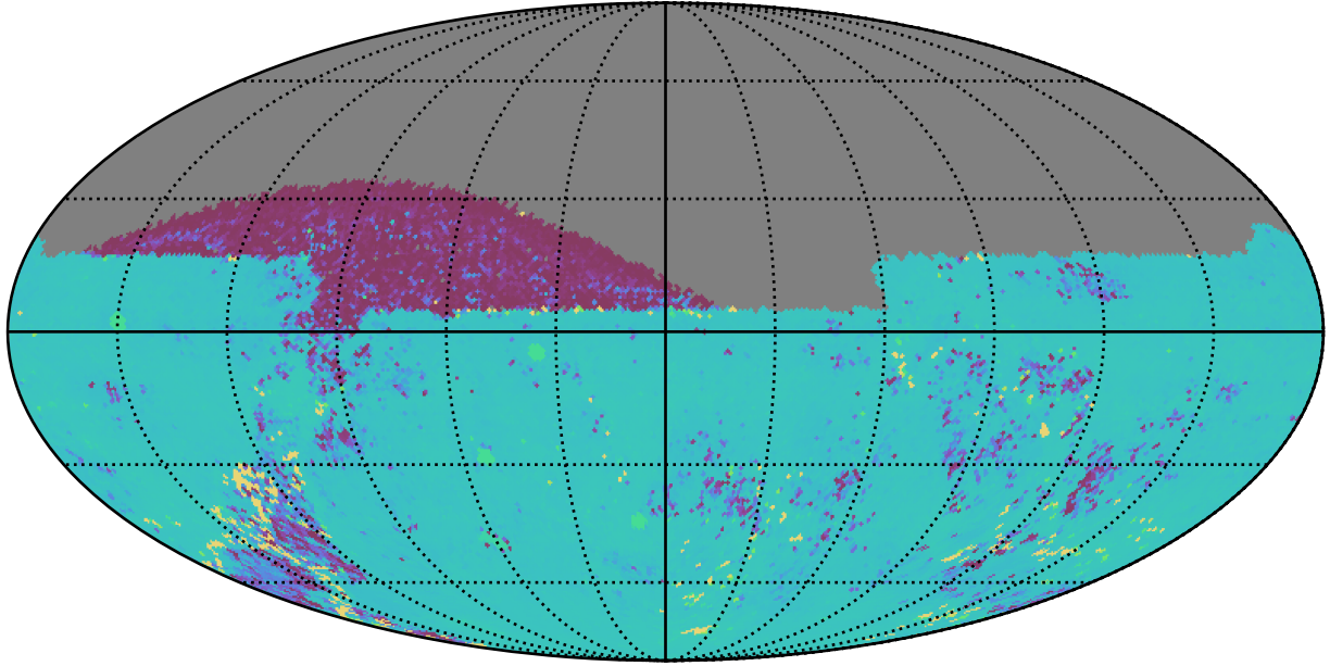
ddf_acor_sf10_lsf40_lsr50_v3.4_10yrs All sky ug bands: 75th Percentile Intranight Timespan
