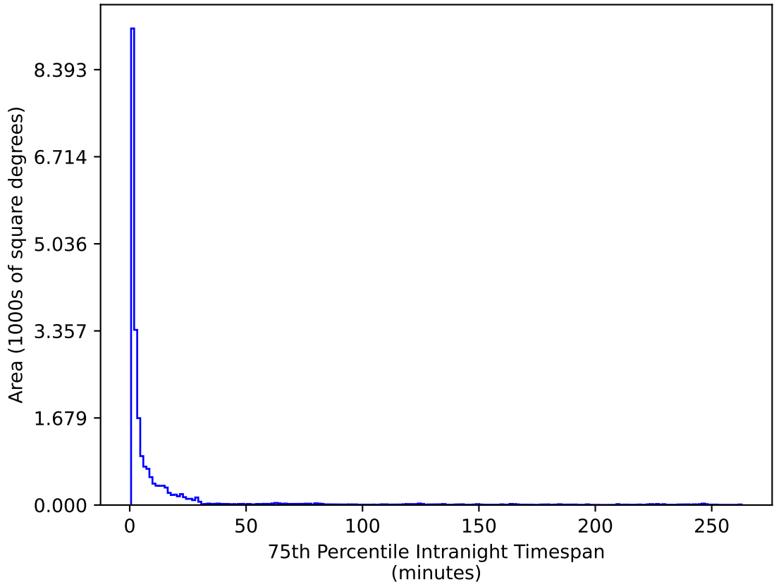
ddf_acor_sf10_lsf40_lsr50_v3.4_10yrs All sky u band: 75th Percentile Intranight Timespan
