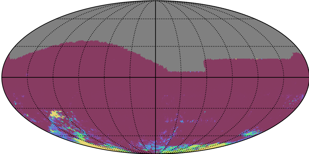
ddf_acor_sf10_lsf40_lsr50_v3.4_10yrs All sky ri bands: 75th Percentile Intranight Timespan
