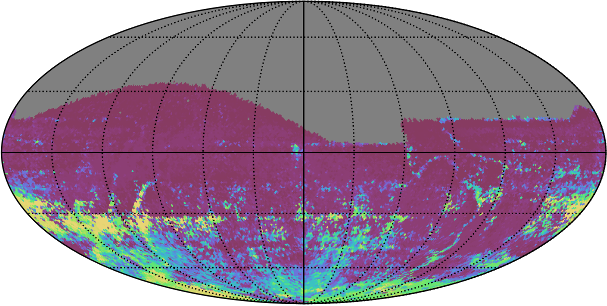
ddf_acor_sf10_lsf40_lsr50_v3.4_10yrs All sky r band: 75th Percentile Intranight Timespan
