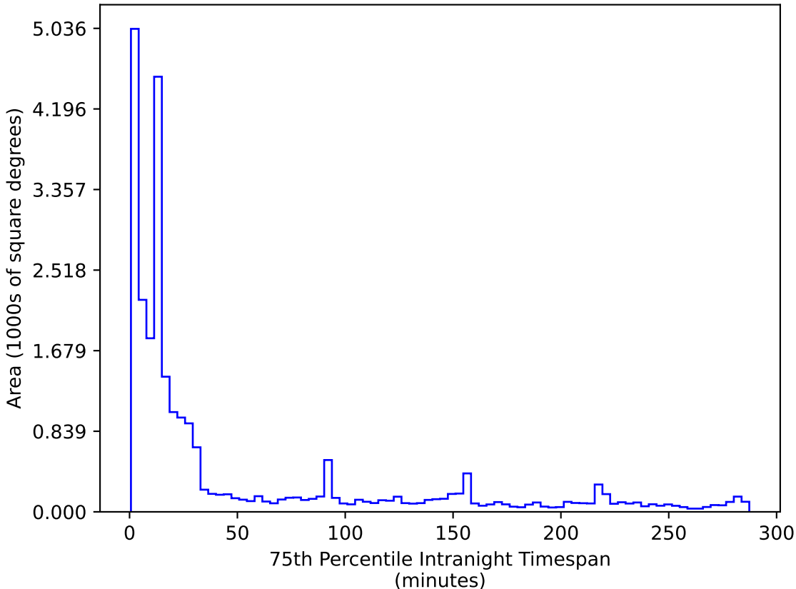
ddf_acor_sf10_lsf40_lsr50_v3.4_10yrs All sky r band: 75th Percentile Intranight Timespan
