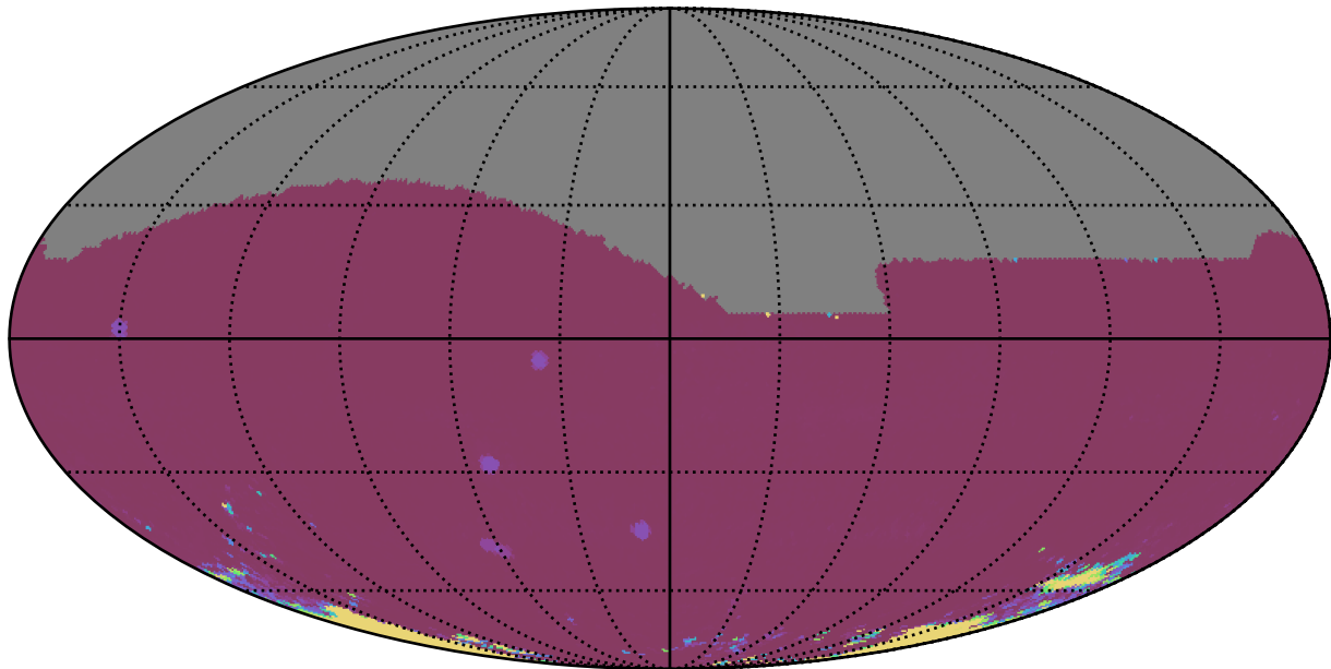
ddf_acor_sf10_lsf40_lsr50_v3.4_10yrs All sky iz bands: 75th Percentile Intranight Timespan
