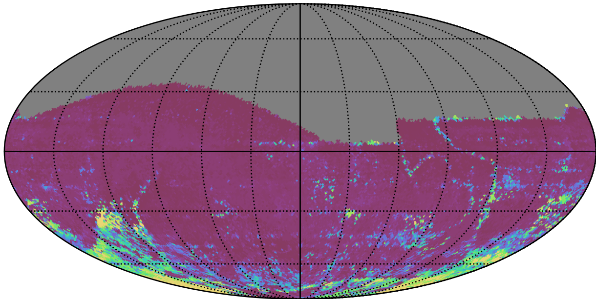
ddf_acor_sf10_ls40_lsr50_v3.4_10yrs All sky i band: 75th Percentile Intranight Timespan
