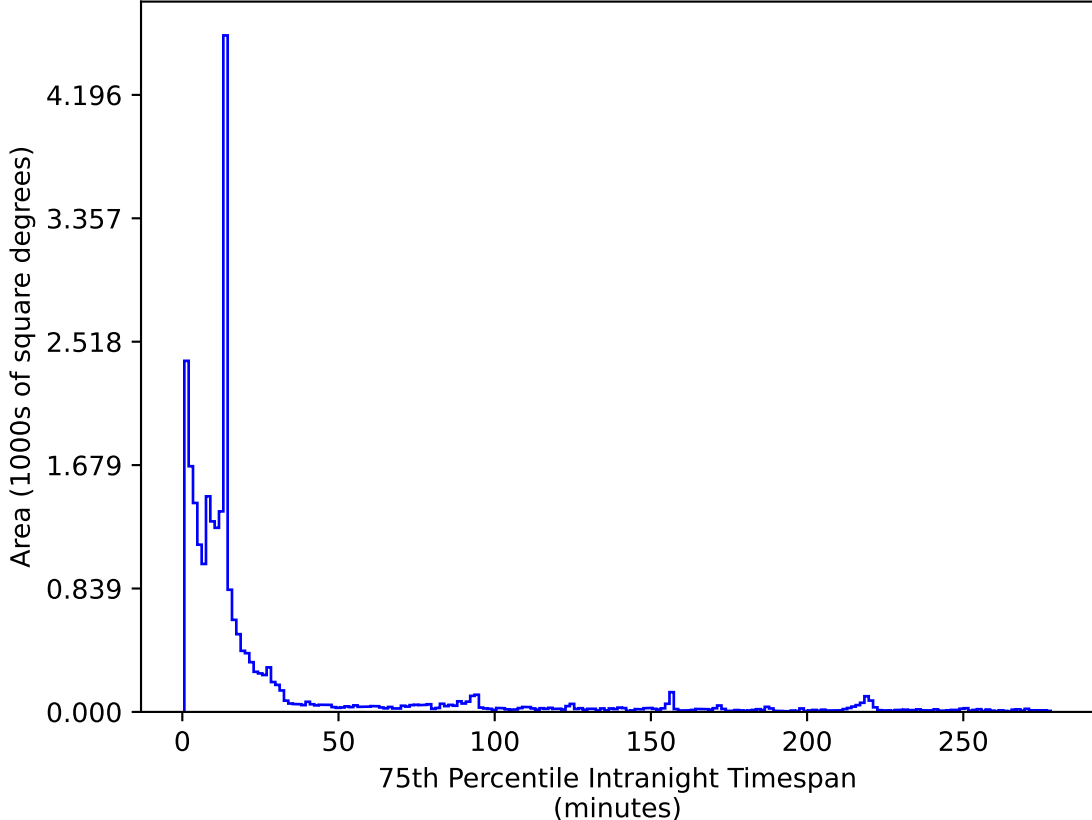
ddf_acor_sf10_lsf40_lsr50_v3.4_10yrs All sky i band: 75th Percentile Intranight Timespan
