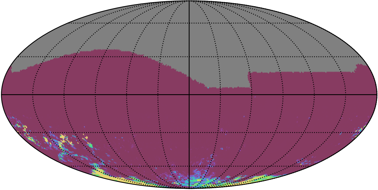
ddf_acor_sf10_lsf40_lsr50_v3.4_10yrs All sky gr bands: 75th Percentile Intranight Timespan
