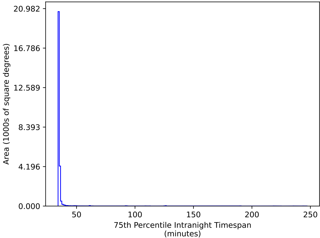
ddf_acor_sf10_lsf40_lsr50_v3.4_10yrs All sky gr bands: 75th Percentile Intranight Timespan
