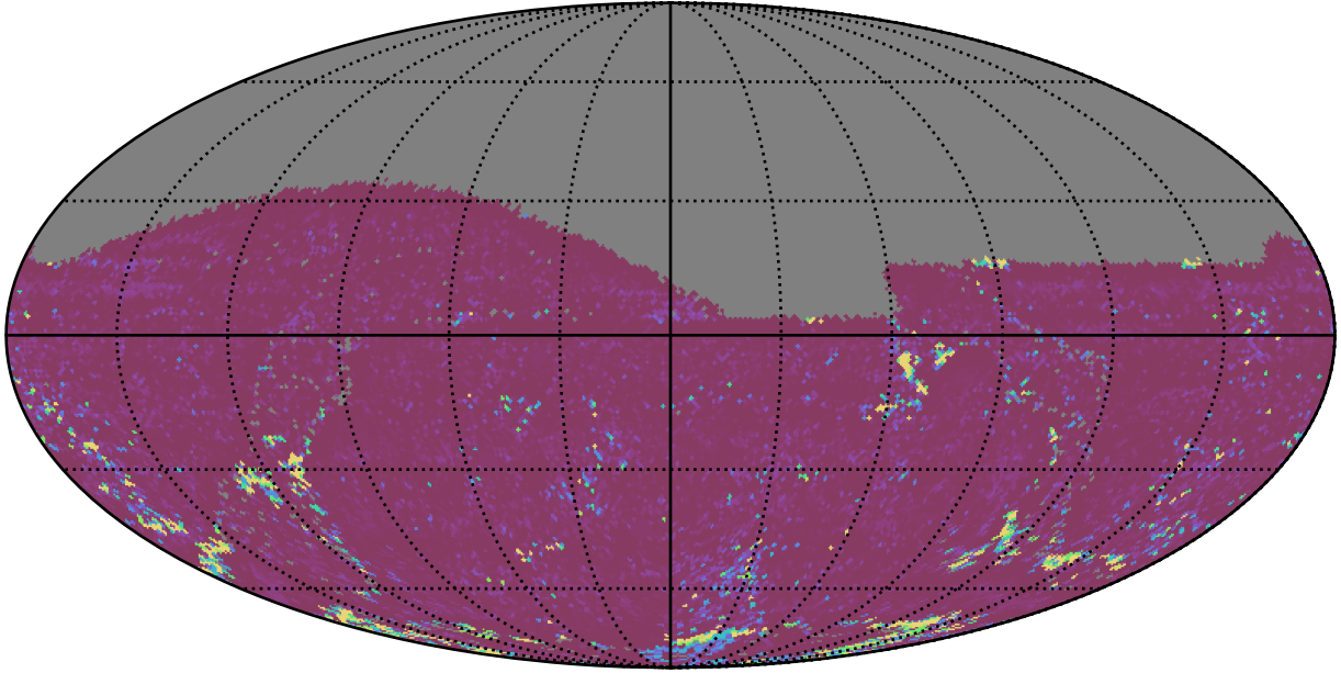
ddf_acor_sf10_lsf40_lsr50_v3.4_10yrs All sky g band: 75th Percentile Intranight Timespan
