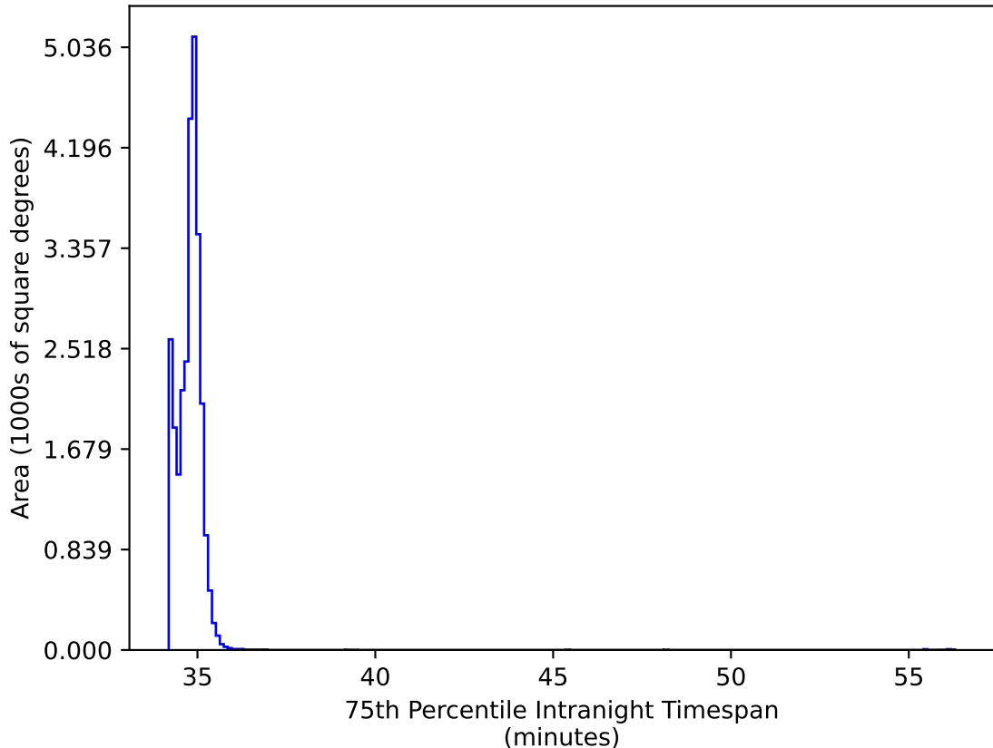
ddf_acor_sf10_lsf40_lsr50_v3.4_10yrs All sky all bands: 75th Percentile Intranight Timespan
