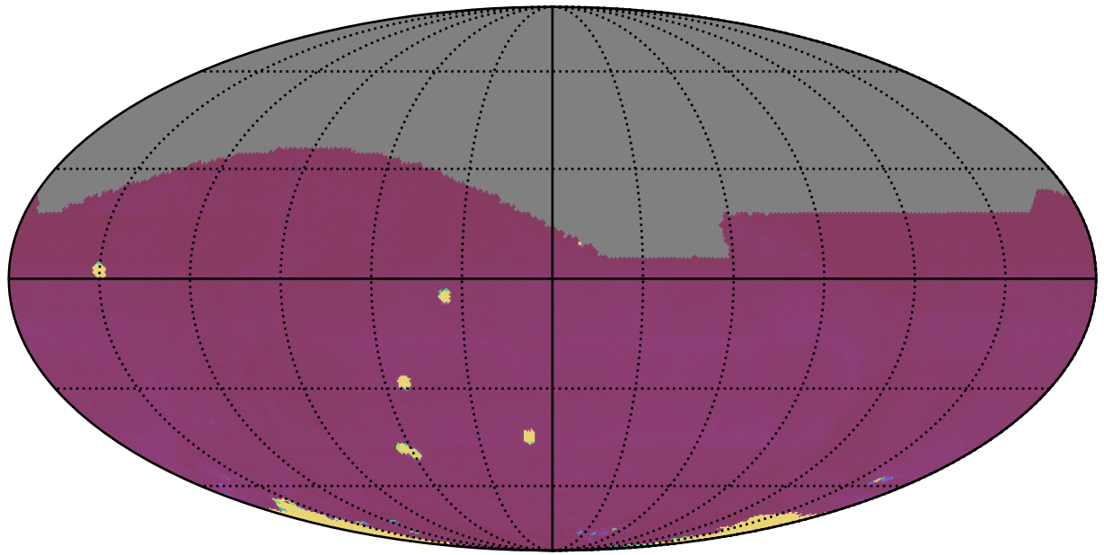
ddf_acor_sf10_lsf40_lsr50_v3.4_10yrs All sky: 75th Percentile Intranight Timespan
