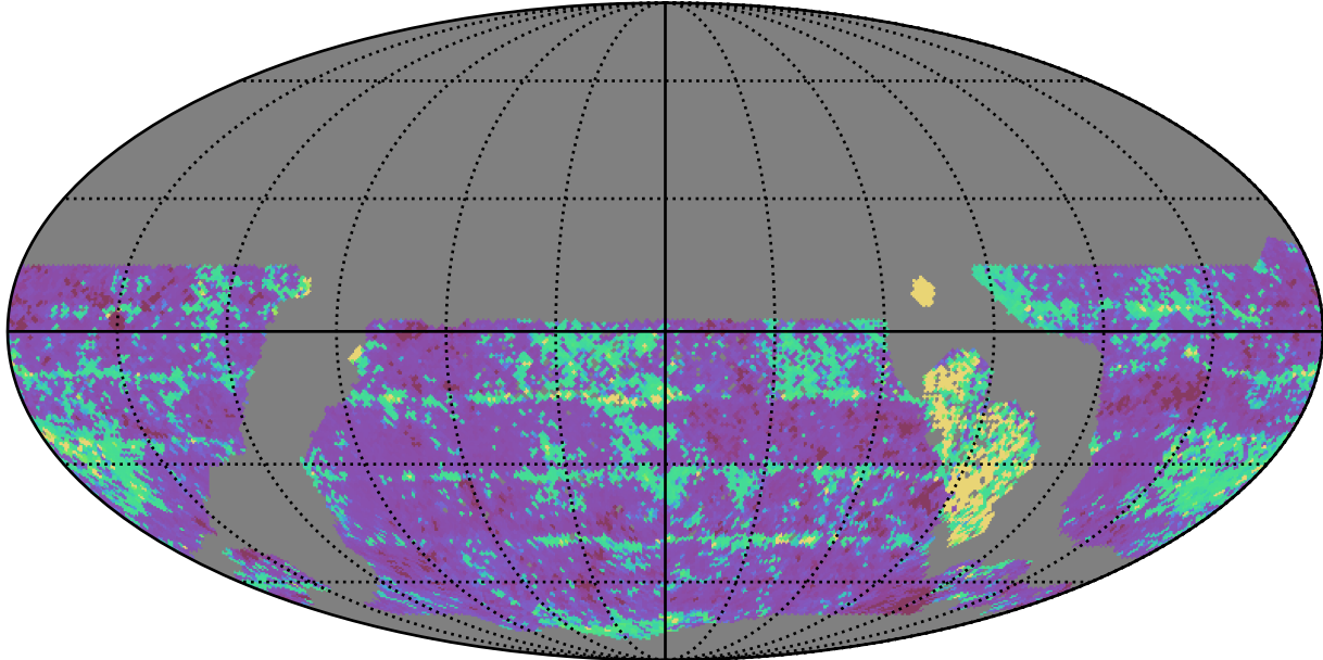
ddf_acor_sf10_lsf40_lsr50_v3.4_10yrs WFD z band: 20thPercentile Inter-Night Gap
