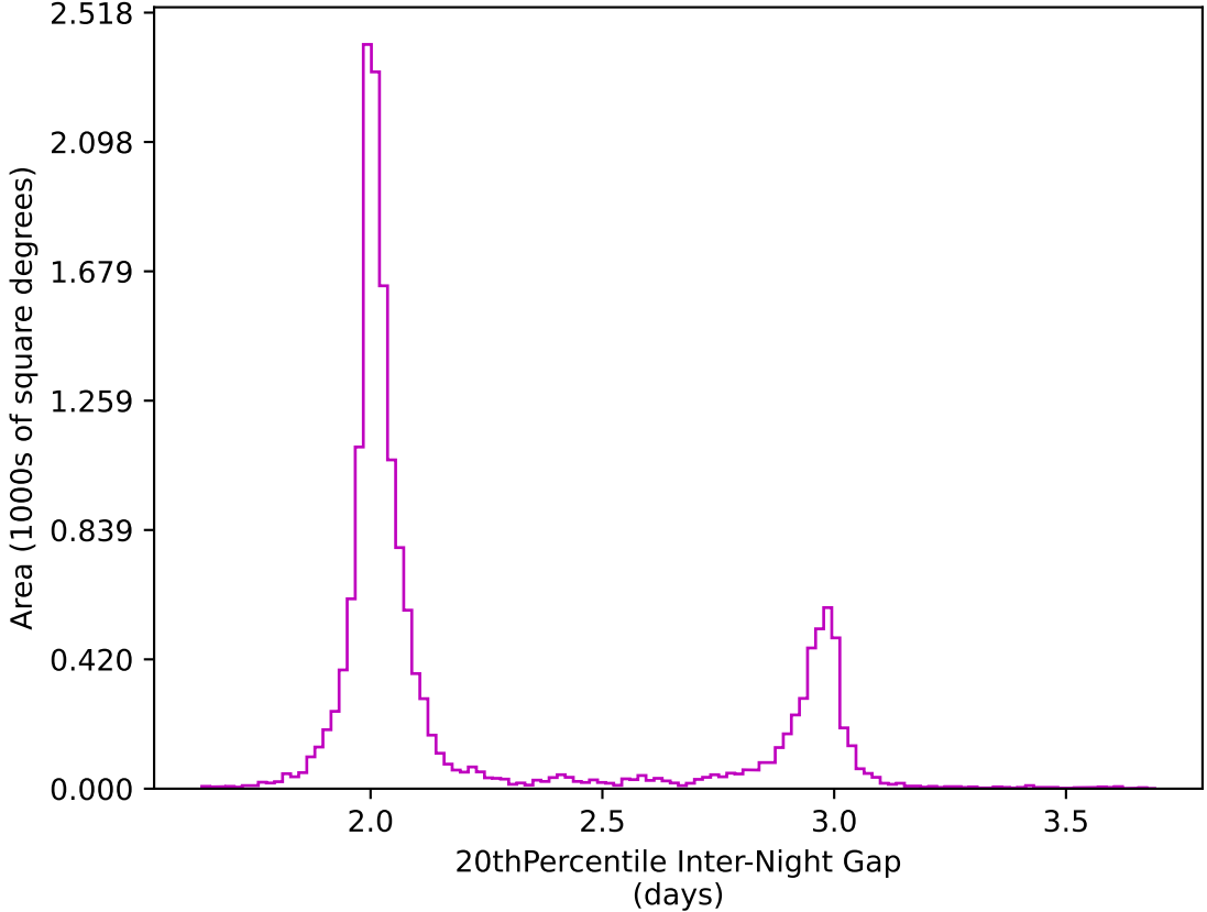
ddf_acor_sf10_lsf40_lsr50_v3.4_10yrs WFD z band: 20thPercentile Inter-Night Gap
