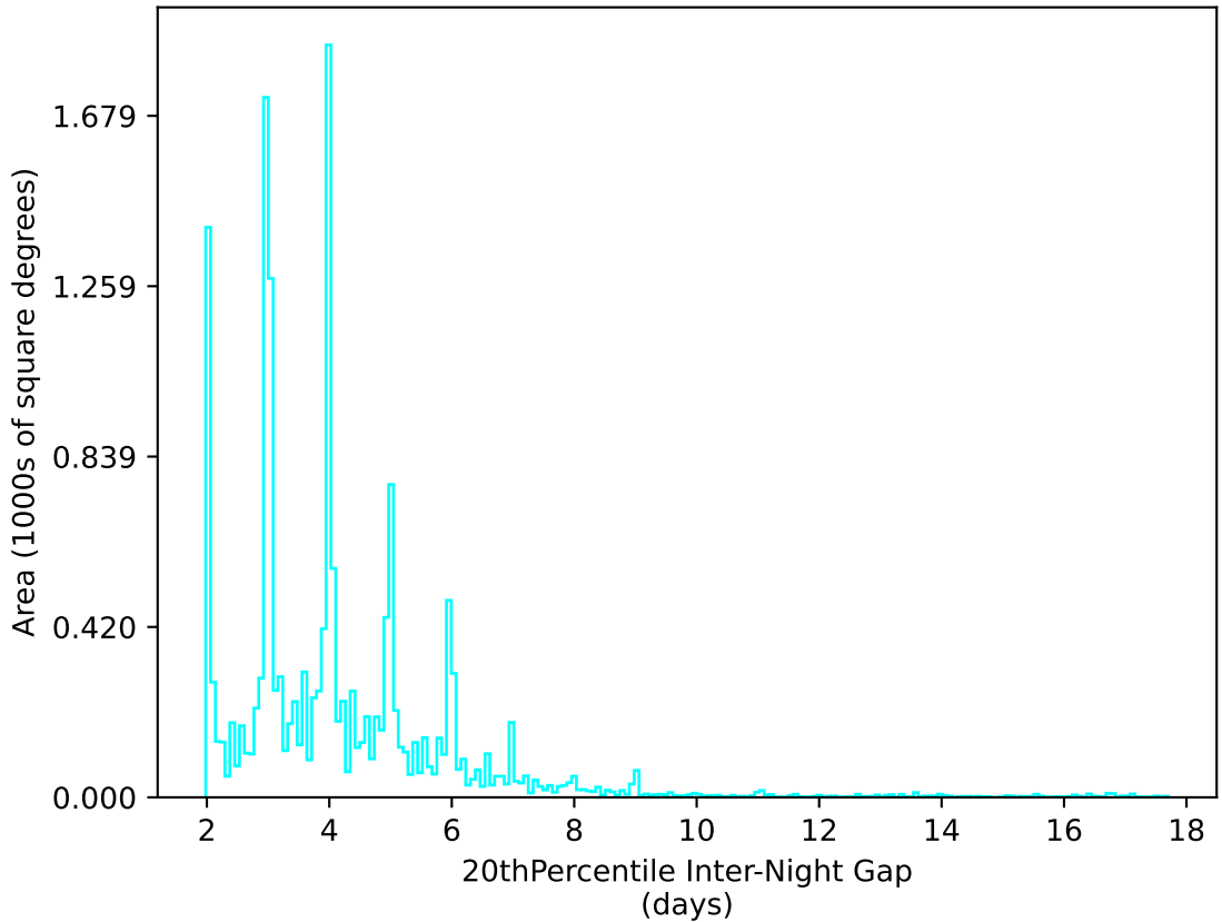
ddf_acor_sf10_ls40_lsr50_v3.4_10yrs WFD u band: 20thPercentile Inter-Night Gap
