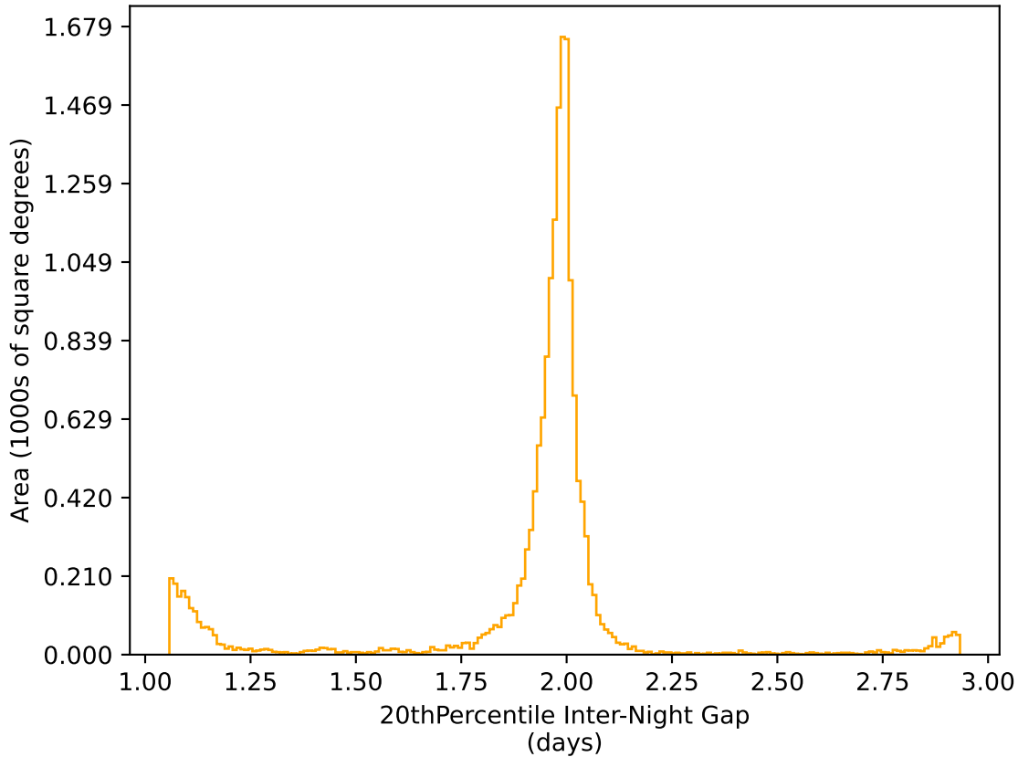
ddf_acor_sf10_lsf40_lsr50_v3.4_10yrs WFD r band: 20thPercentile Inter-Night Gap
