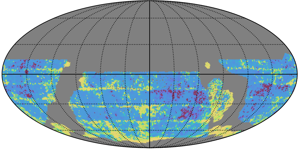
ddf_acor_sf10_lsf40_lsr50_v3.4_10yrs WFD i band: 20thPercentile Inter-Night Gap
