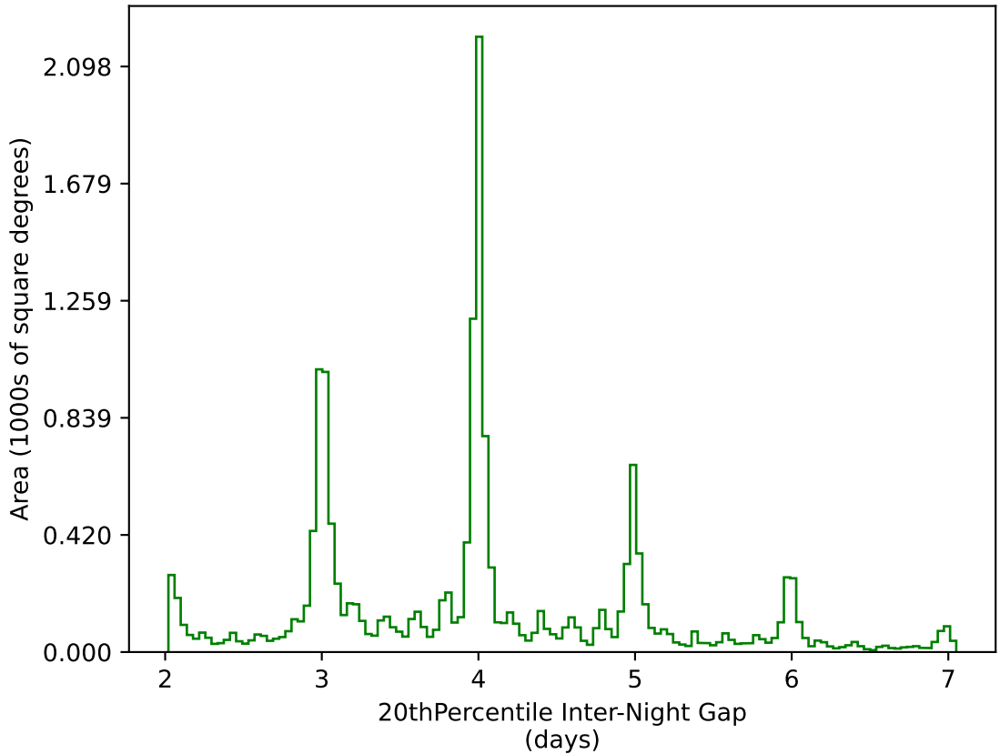
ddf_acor_sf10_lsf40_lsr50_v3.4_10yrs WFD g band: 20thPercentile Inter-Night Gap
