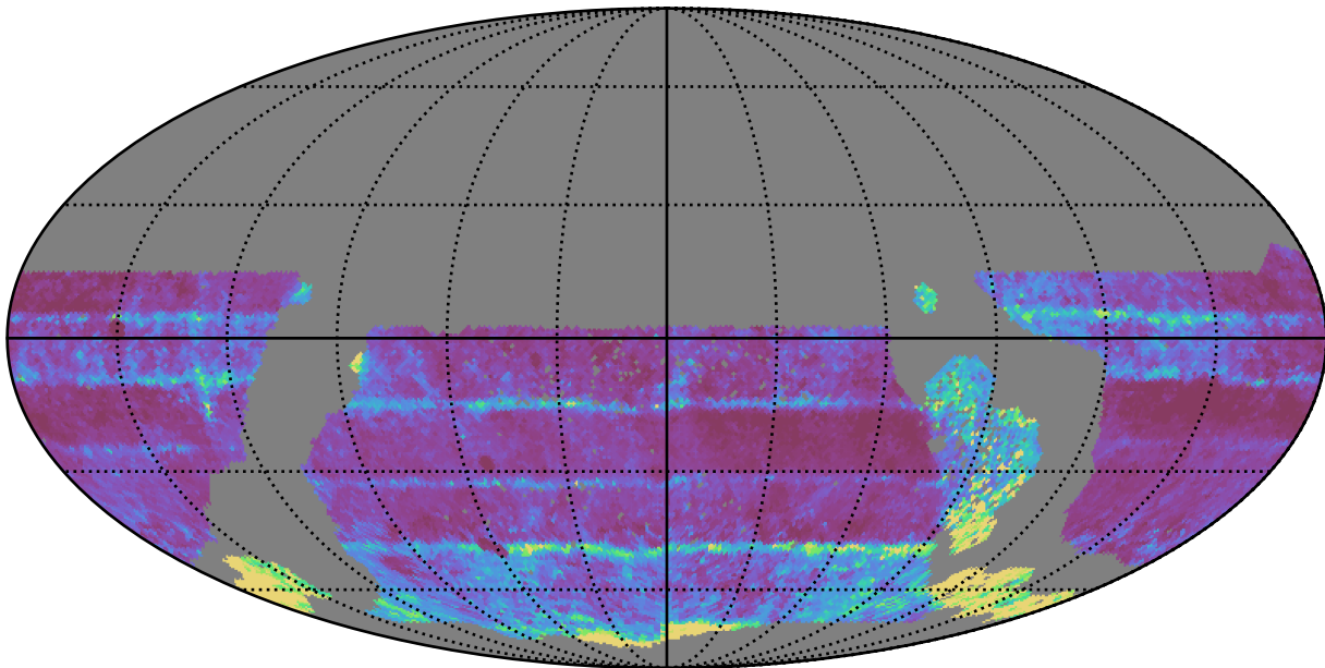
ddf_acor_sf10_lsf40_lsr50_v3.4_10yrs WFD all bands: 20thPercentile Inter-Night Gap
