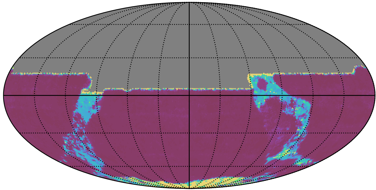
ddf_acor_sf10_lsf40_lsr50_v3.4_10yrs All sky y band: 20thPercentile Inter-Night Gap
