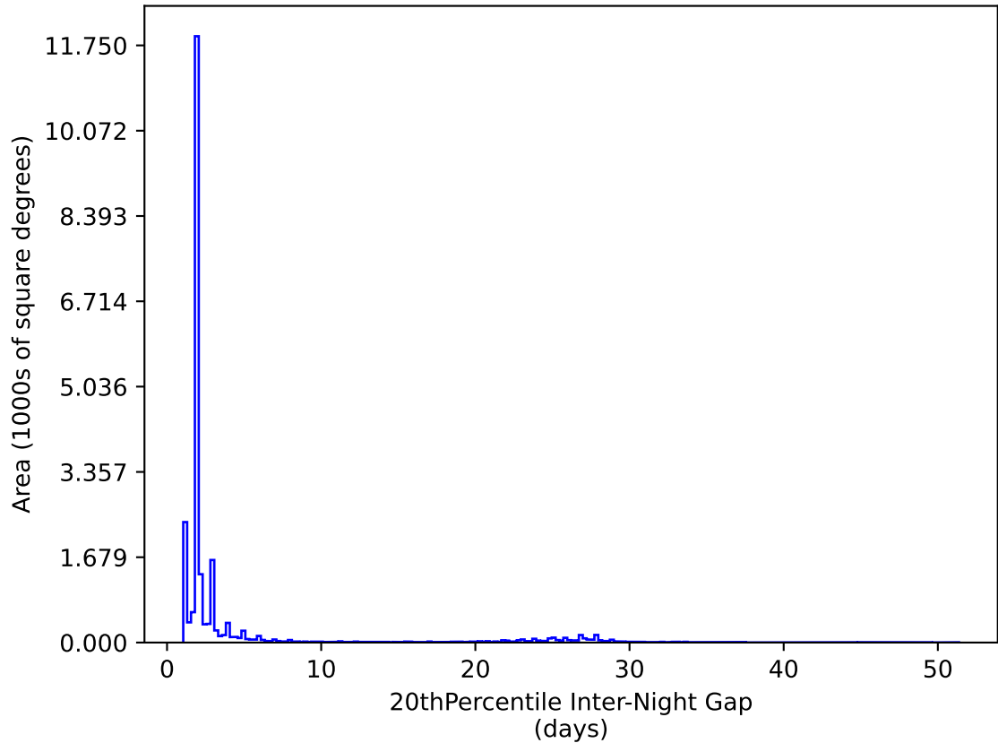
ddf_acor_sf10_lsf40_lsr50_v3.4_10yrs All sky y band: 20thPercentile Inter-Night Gap
