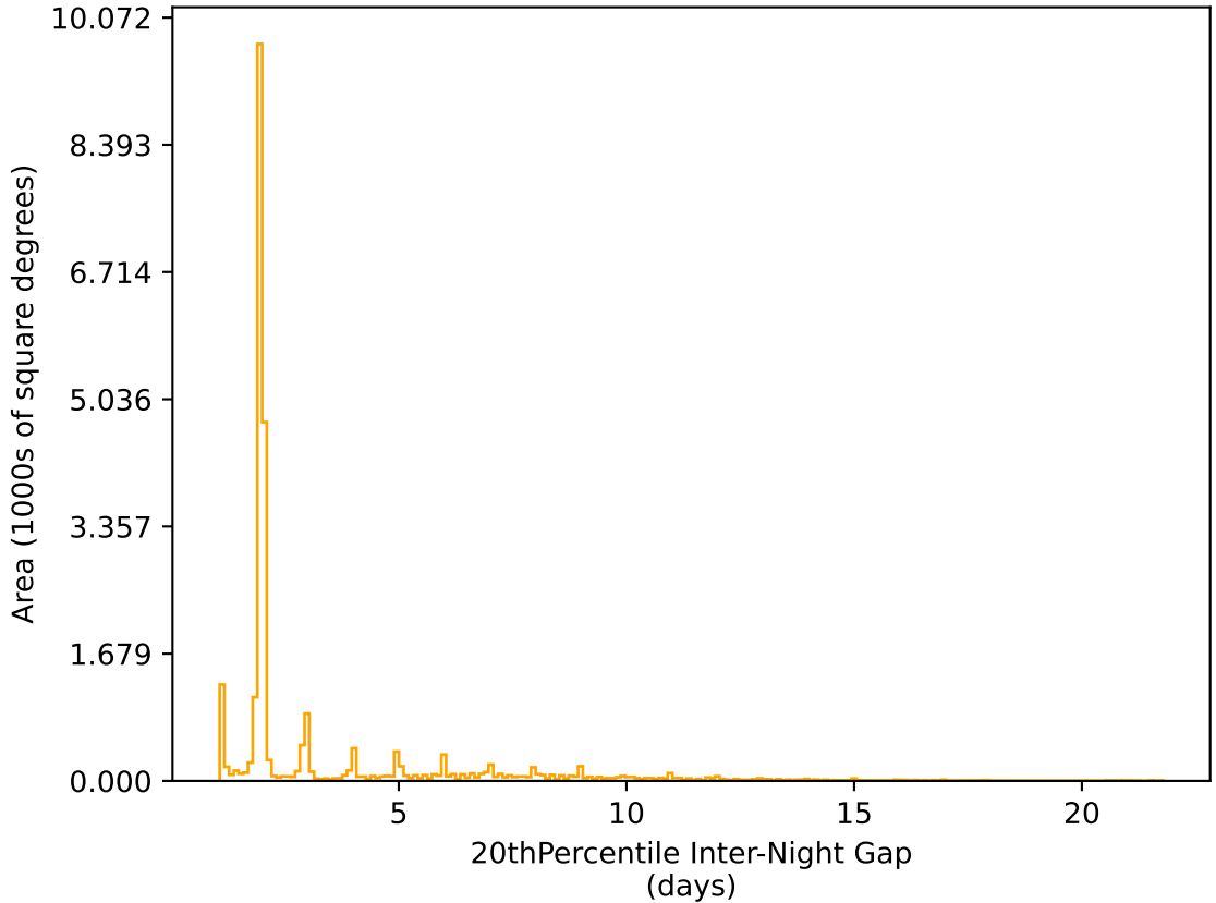
ddf_acor_sf10_lsf40_lsr50_v3.4_10yrs All sky r band: 20thPercentile Inter-Night Gap
