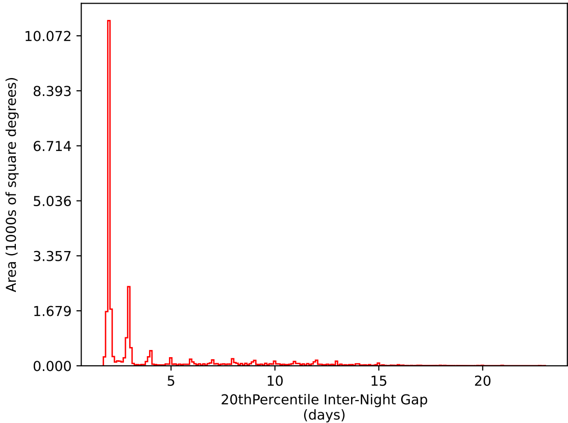
ddf_acor_sf10_ls40_lsr50_v3.4_10yrs All sky i band: 20thPercentile Inter-Night Gap
