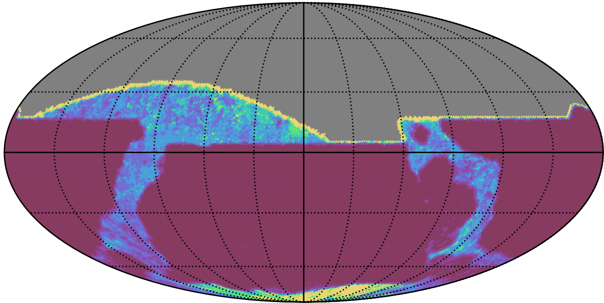
ddf_acor_sf10_lsf40_lsr50_v3.4_10yrs All sky all bands: 20thPercentile Inter-Night Gap
