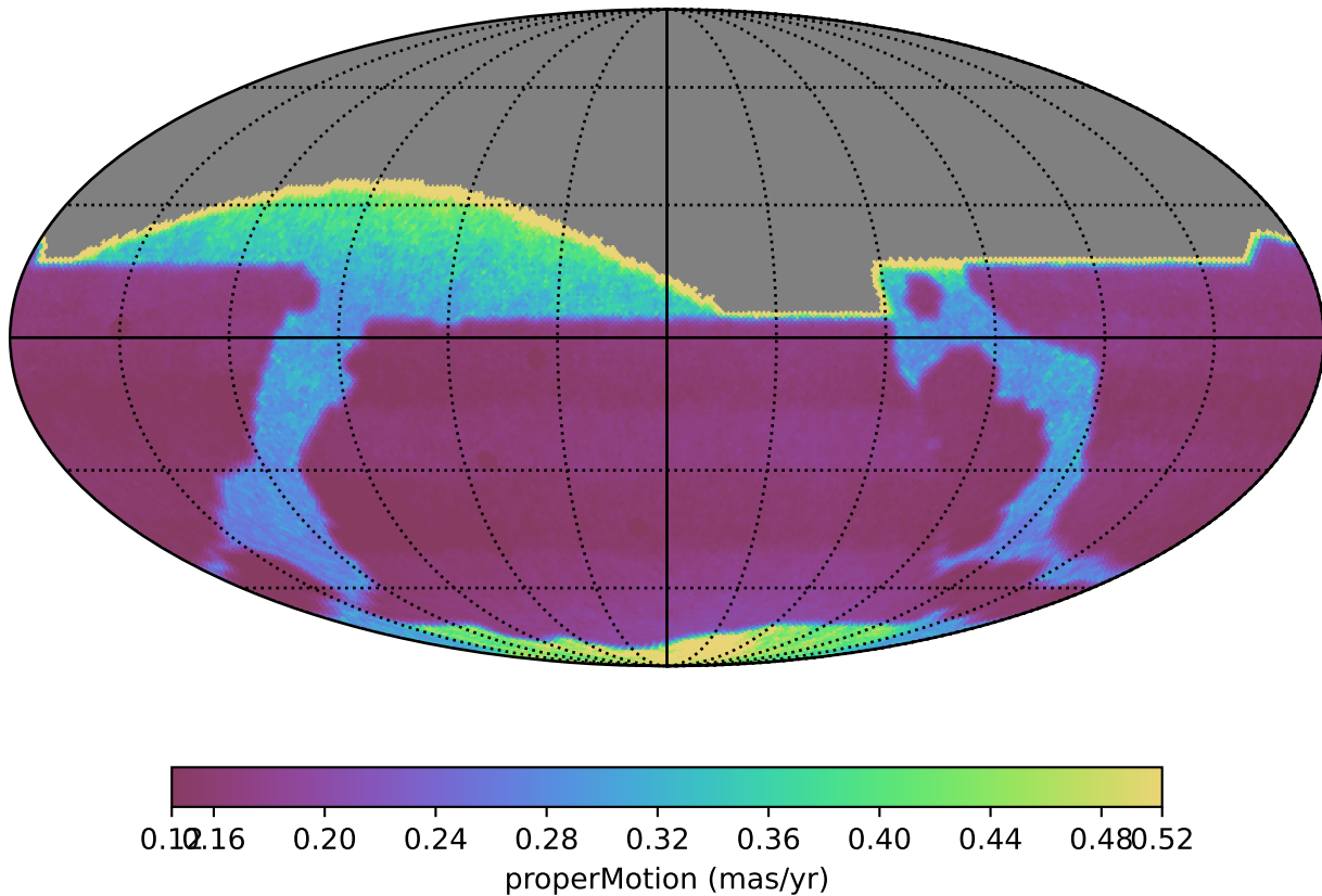
ddf_acor_sf10_lsf40_lsr50_v3.4_10yrs : properMotion
