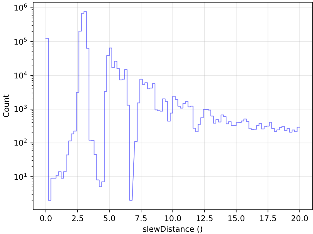
ddf_acor_sf10_lsf40_lsr50_v3.4_10yrs All visits: Zoom Slew Distance Histogram
