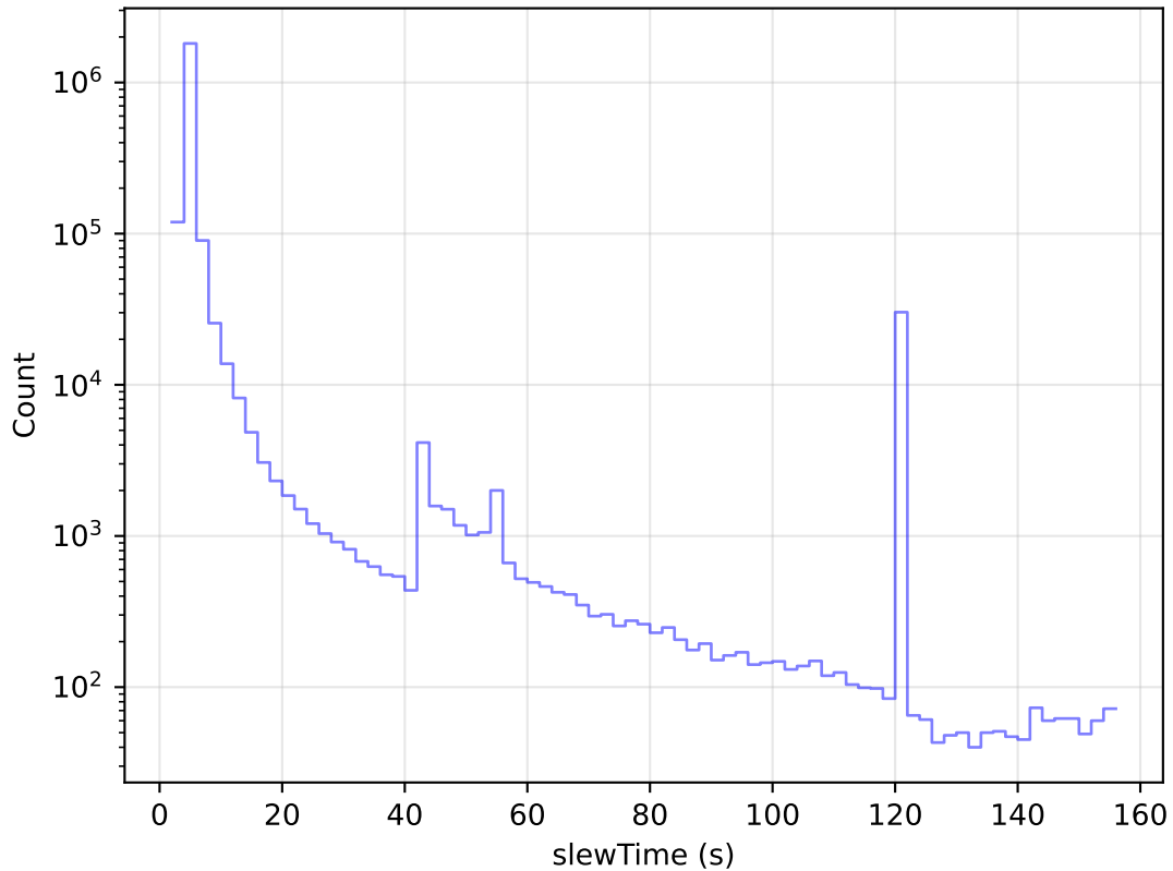
ddf_acor_sf10_lsf40_lsr50_v3.4_10yrs All visits: Slew Time Histogram
