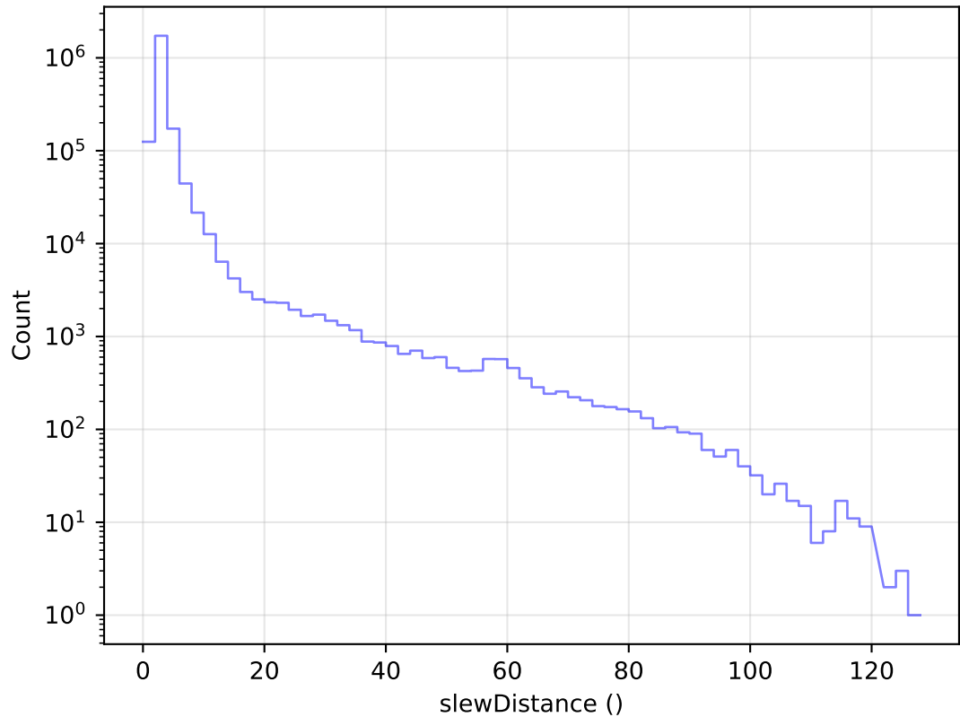
ddf_acor_sf10_lsf40_lsr50_v3.4_10yrs All visits: Slew Distance Histogram
