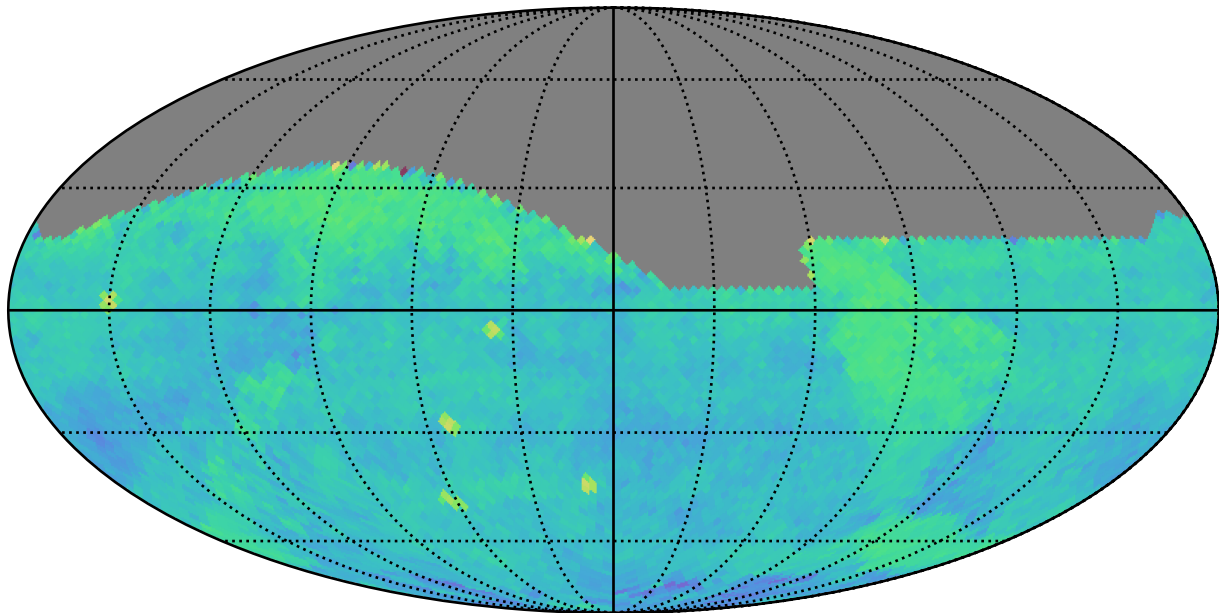
ddf_acor_sf10_lsf40_lsr50_v3.4_10yrs (g or r or i): PairFraction
