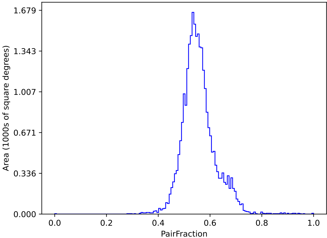
ddf_acor_sf10_lsf40_lsr50_v3.4_10yrs (g or r or i): PairFraction
