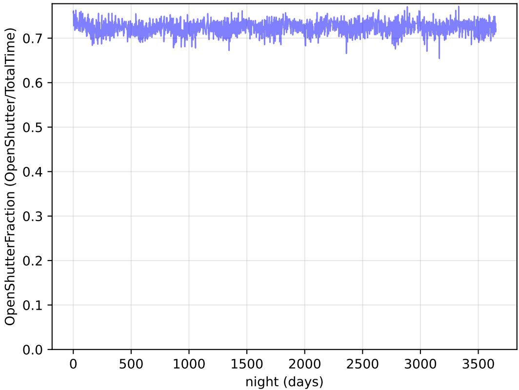
ddf_acor_sf10_lsf40_lsr50_v3.4_10yrs : OpenShutterFraction
