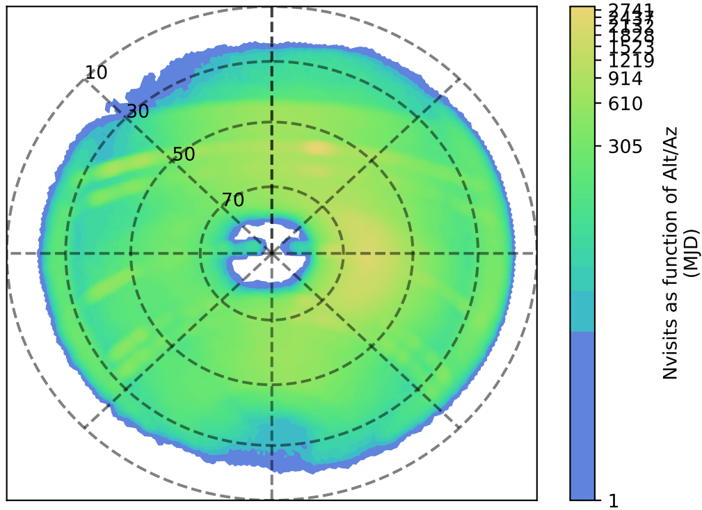
ddf_acor_sf10_lsf40_lsr50_v3.4_10yrs z: Nvisits as function of Alt/Az
