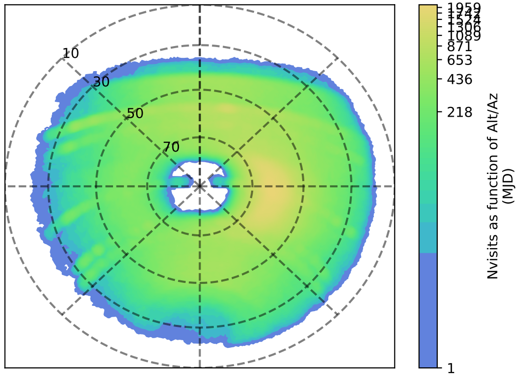
ddf_acor_sf10_lsf40_lsr50_v3.4_10yrs y: Nvisits as function of Alt/Az
