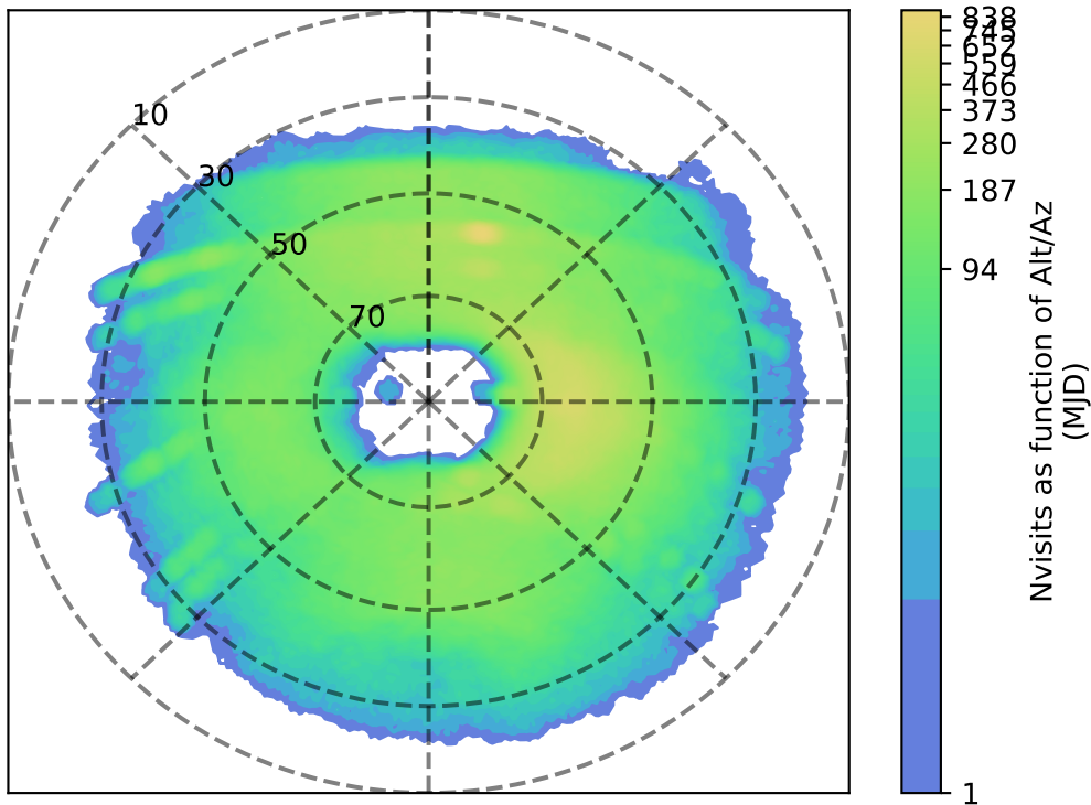
ddf_acor_sf10_lsf40_lsr50_v3.4_10yrs u: Nvisits as function of Alt/Az
